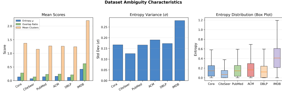
Figure 7: Dataset ambiguity characteristics. (Left) Mean entropy, overlap ratio, and cluster count per dataset. IMDB stands out with the highest entropy and overlap ratio. (Center) Entropy standard deviation. (Right) Entropy distribution box plots. IMDB shows the widest distribution, explaining why it benefits most from adaptive thresholding.
