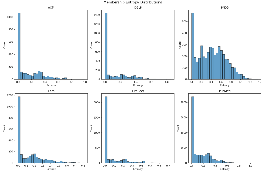
Figure 11: Membership entropy distributions for each dataset. IMDB shows the widest distribution (highest variance), explaining why it benefits most from adaptive thresholding. CiteSeer shows the narrowest distribution concentrated near zero.
