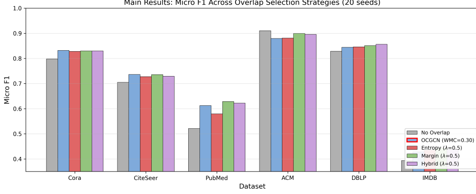
Fig. 2 Micro F1 scores across all overlap selection strategies (20 seeds). Bars with red outlines indicate the best result per dataset. Adaptive methods are competitive with or outperform the fixed WMC default on most datasets; on ACM the no-overlap configuration is best.
