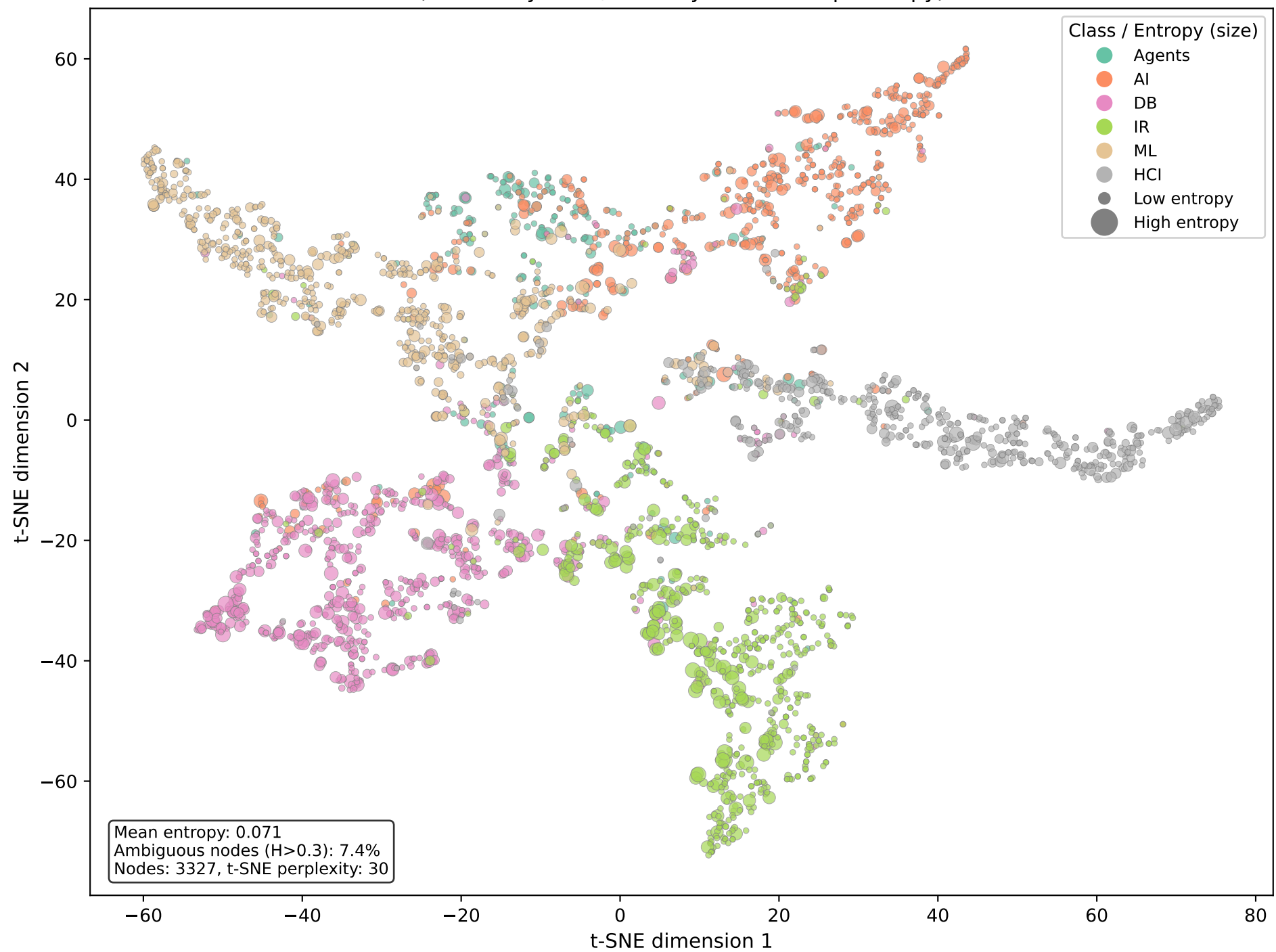
t-SNE Visualization of GCN Embeddings — CiteSeer (colored by class, sized by membership entropy)
