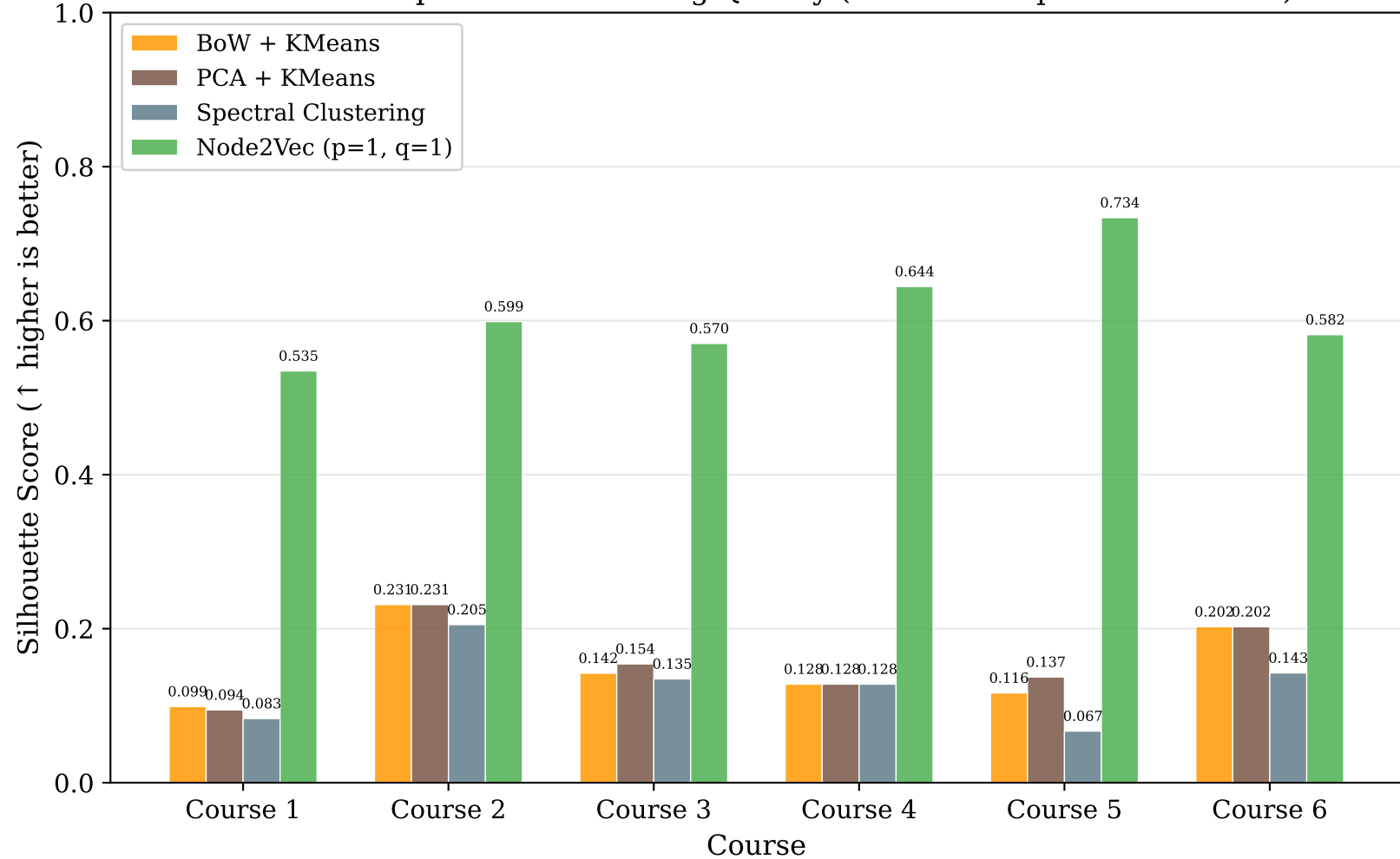
Method Comparison: Clustering Quality (Revised Graph Construction)
