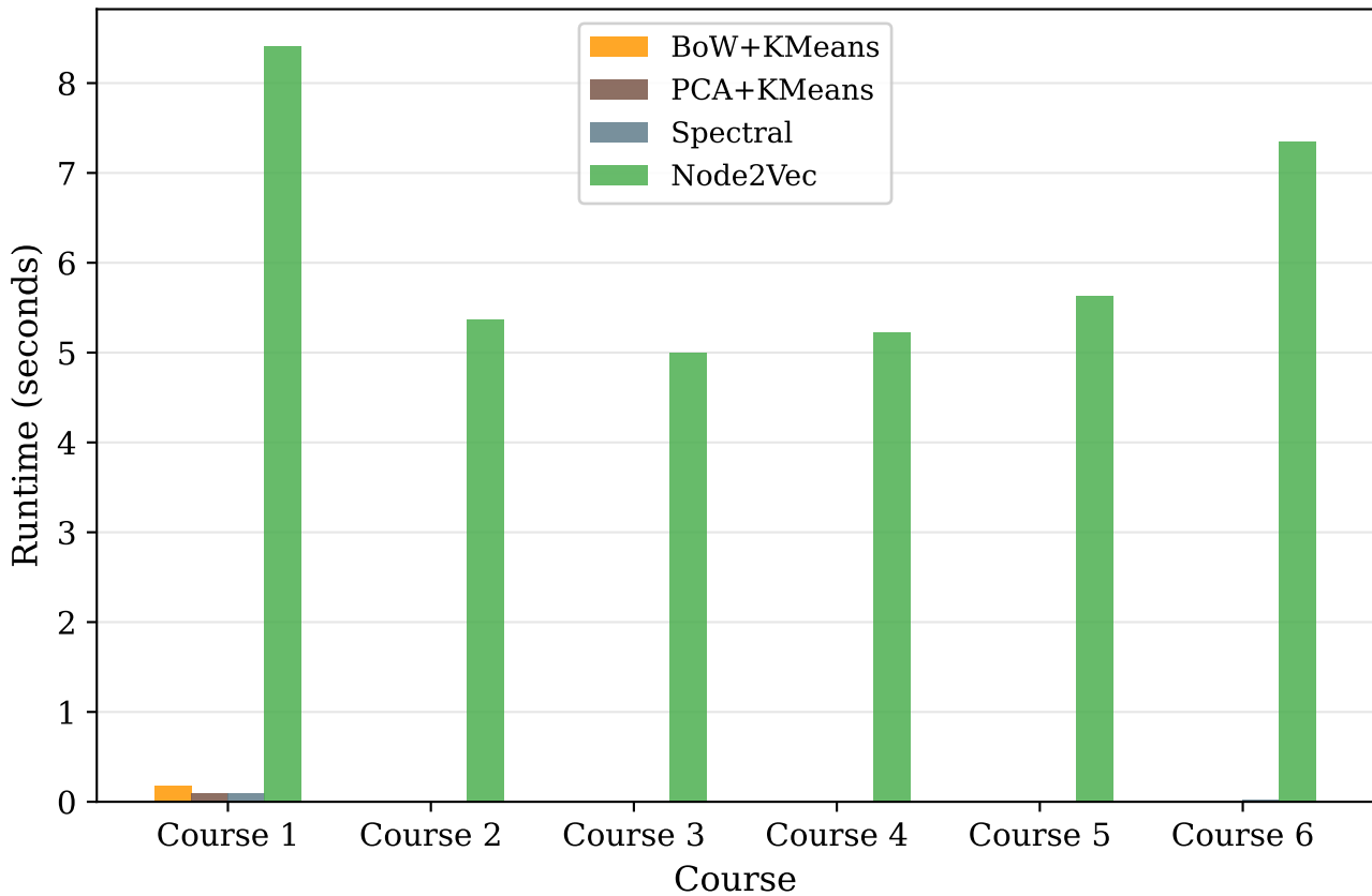
Runtime Comparison Across Methods
