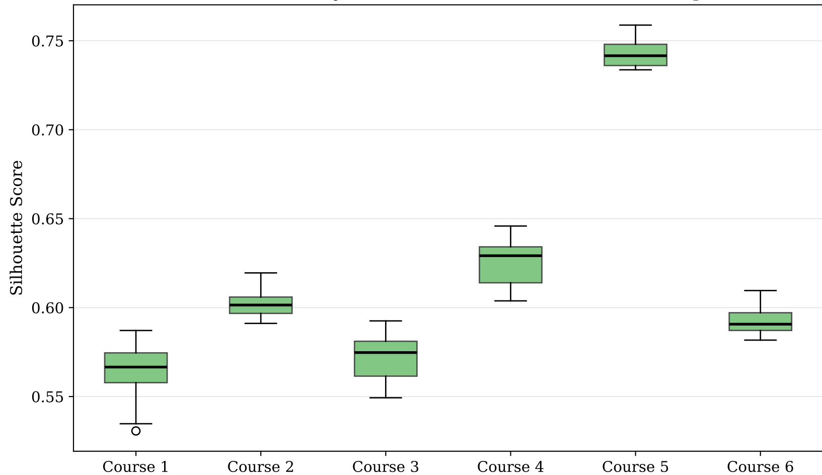
Node2Vec Stability Across 20 Random Seeds (Revised Graph)
