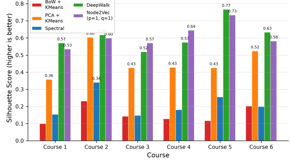
Fig. 4: Silhouette scores ( \uparrow higher is better) for five student sectioning methods across six courses: BoW + KMeans, PCA + KMeans, Spectral Clustering, DeepWalk (unbiased random walk), and Node2Vec ( p=1 , q=1 ).
