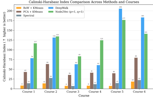
Fig. 8: Calinski–Harabasz Index ( \uparrow higher is better) across the six courses for different clustering methods and representations.
