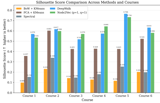
Fig. 6: Silhouette score ( \uparrow higher is better) comparison across the six courses for different clustering algorithms applied to the conventional Student-Course representation and Node2Vec embeddings.
