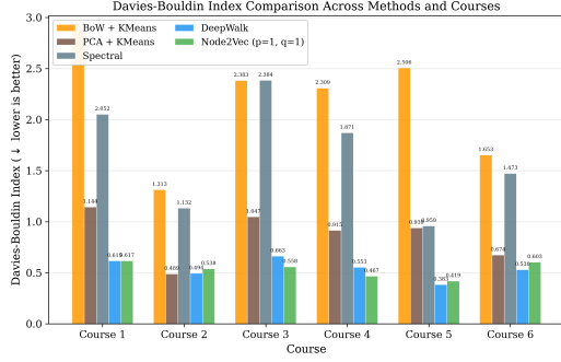
Fig. 7: Davies–Bouldin Index ( \downarrow lower is better) across the six courses for different clustering methods and representations.
