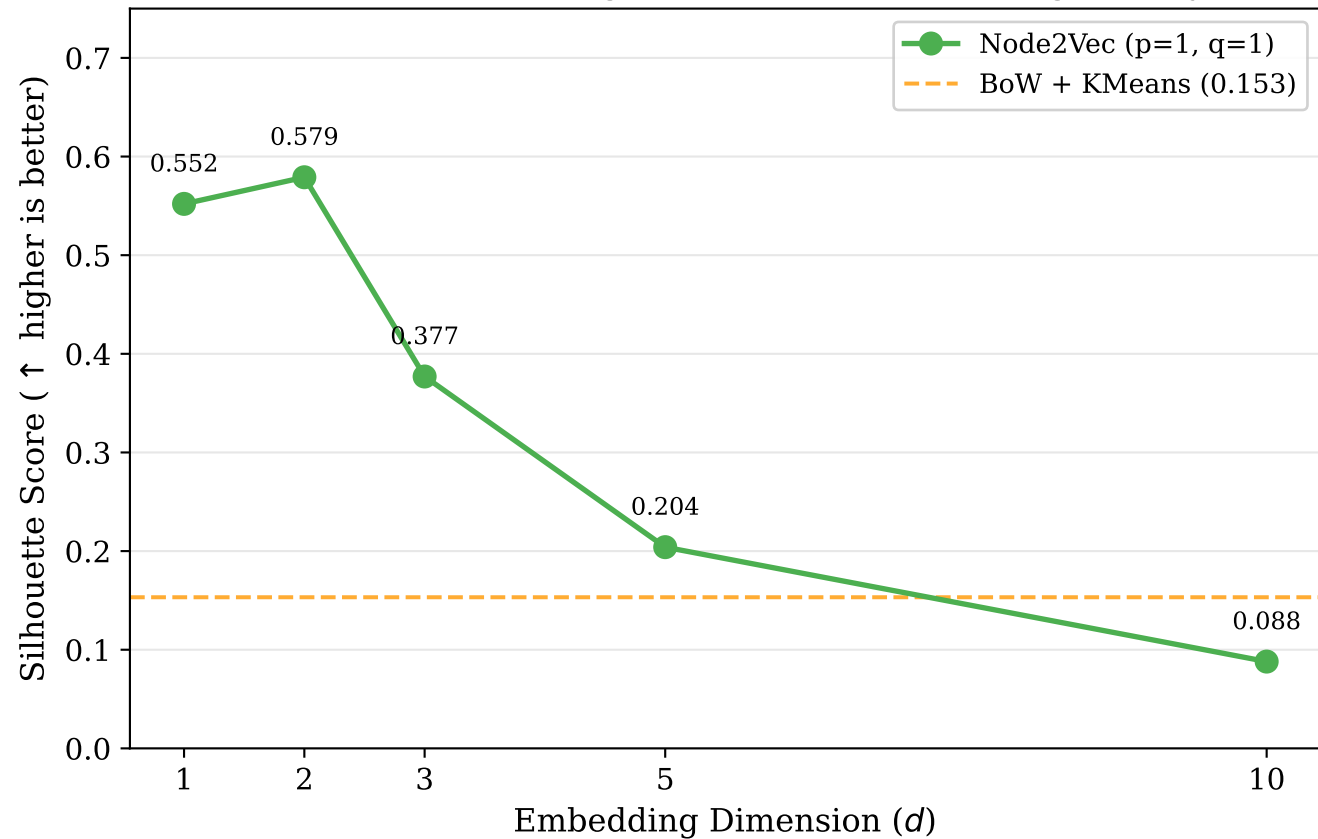
Impact of Embedding Dimension on Clustering Quality
