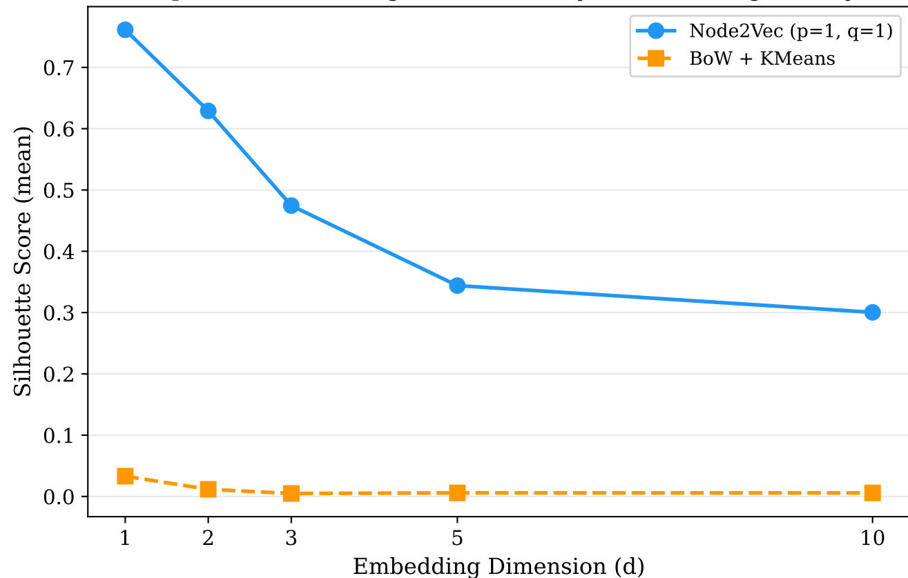
Impact of Embedding Dimensionality on Clustering Quality
