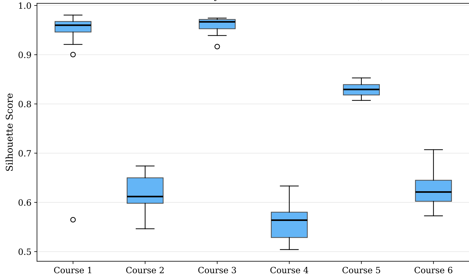
Node2Vec Stability Across 20 Random Seeds (d=1)
