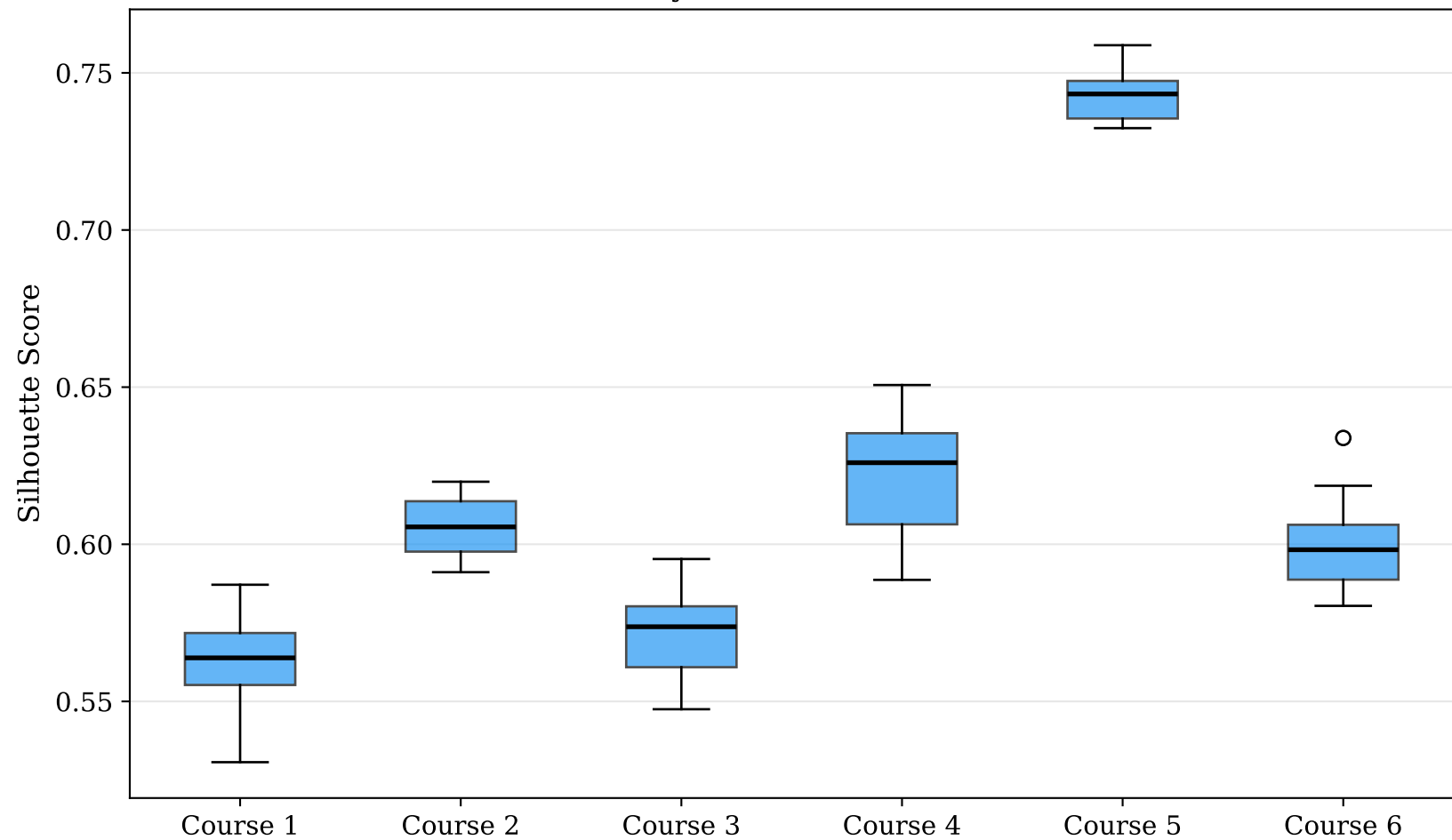
Node2Vec Stability Across 20 Random Seeds (d=2)
