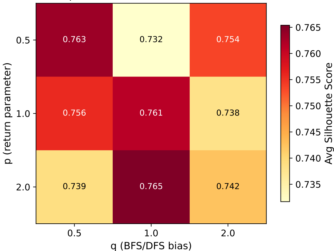
Node2Vec Sensitivity — d=1 (Independent color scale: [0.732, 0.765])
