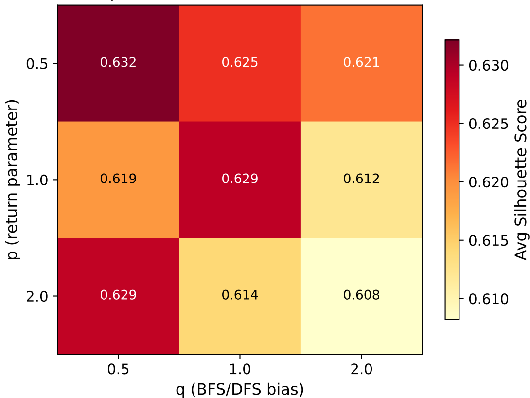
Node2Vec Sensitivity — d=2 (Independent color scale: [0.608, 0.632])
