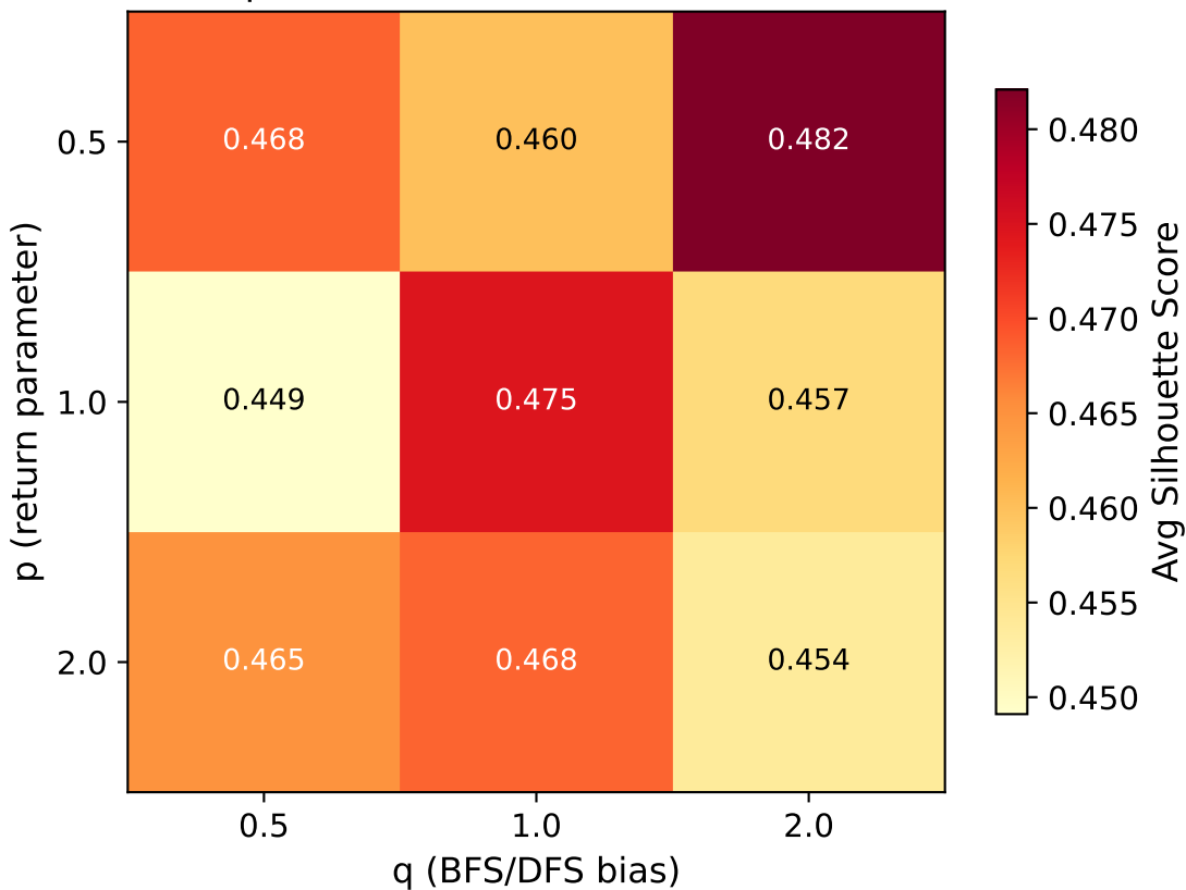
Node2Vec Sensitivity — d=3 (Independent color scale: [0.449, 0.482])
