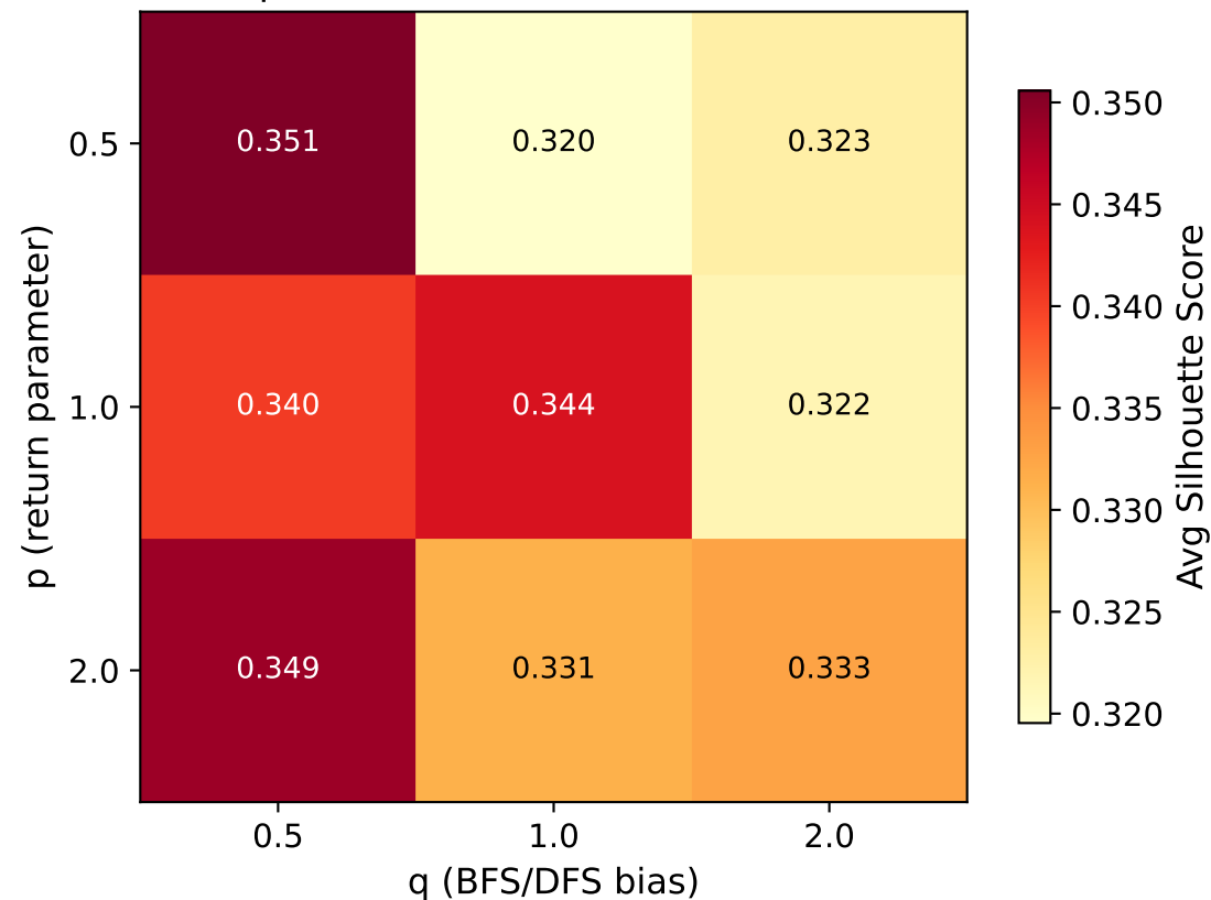
Node2Vec Sensitivity — d=5 (Independent color scale: [0.320, 0.351])
