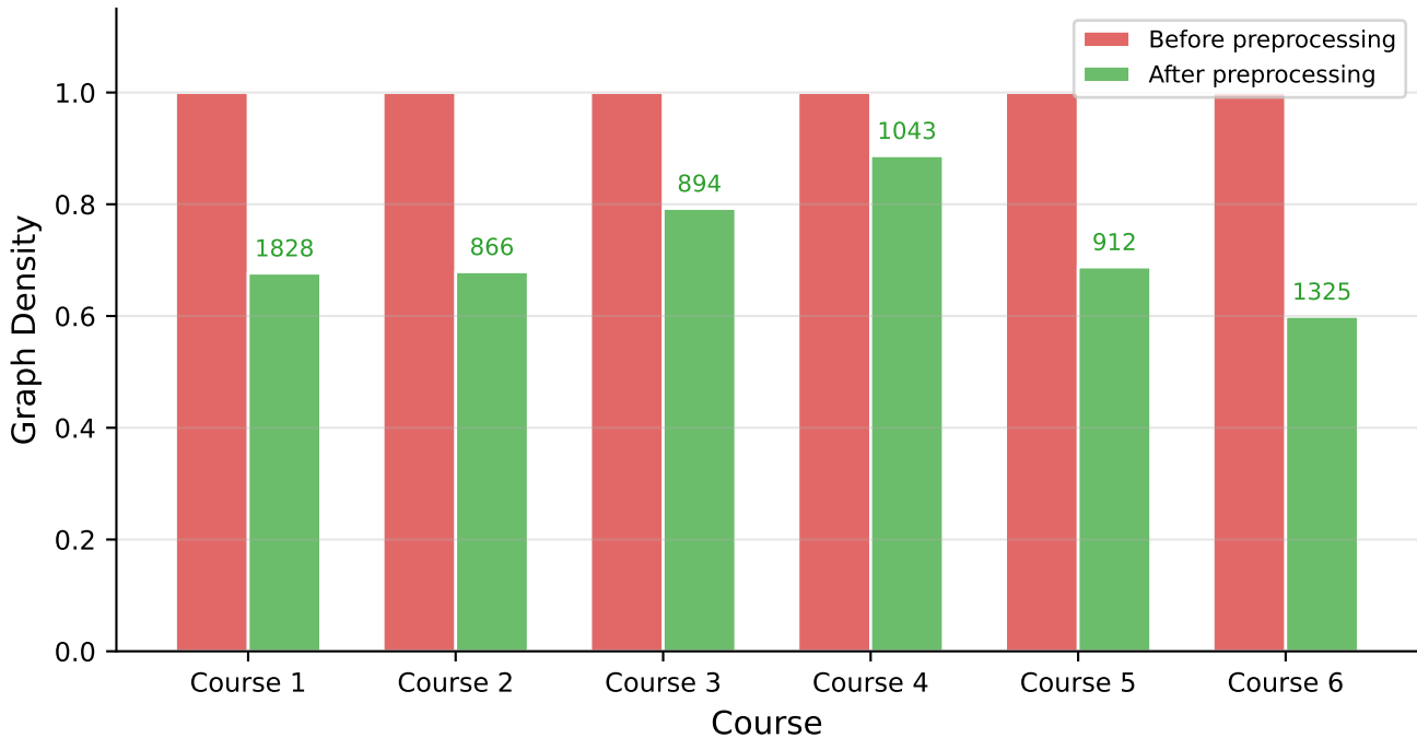
Effect of Constant-Course Removal on Graph Density
