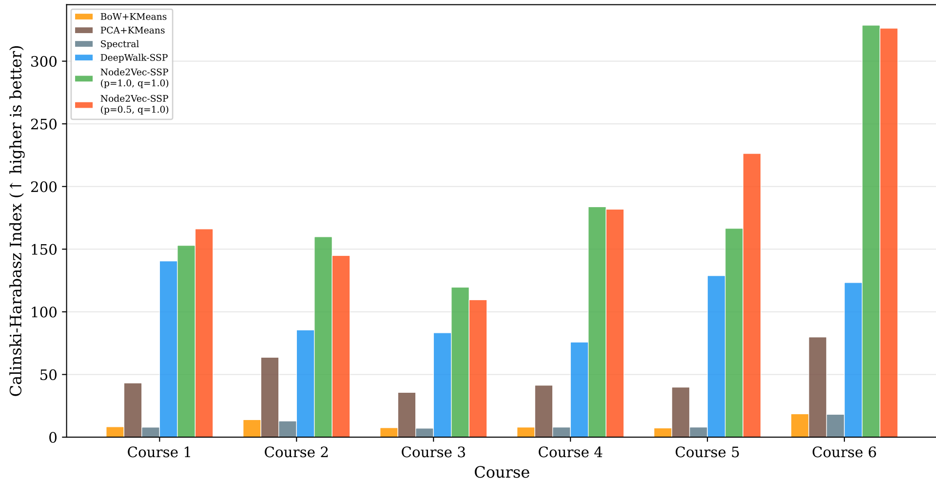
Calinski-Harabasz Index Across Six Courses
