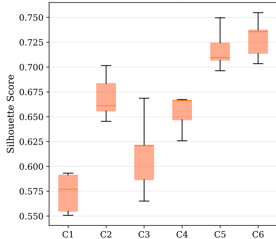
Node2Vec(0.5,1) Seed Stability (n=5)
