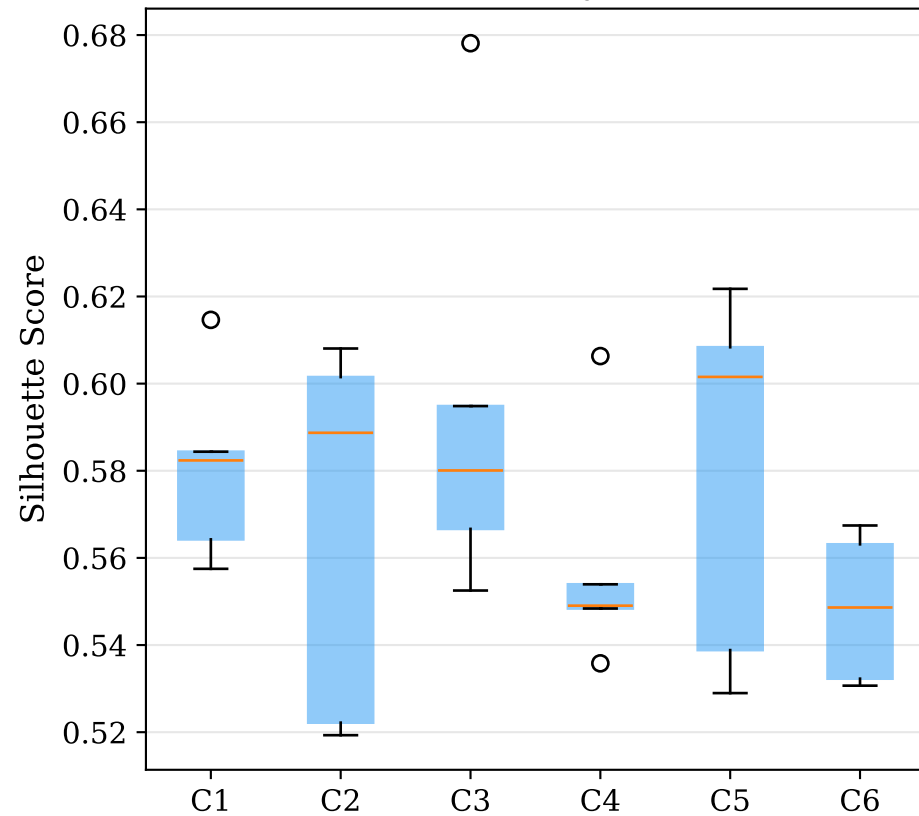
DeepWalk Seed Stability (n=5)
