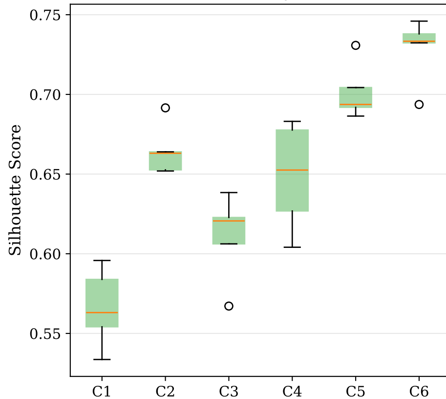
Node2Vec(1,1) Seed Stability (n=5)
