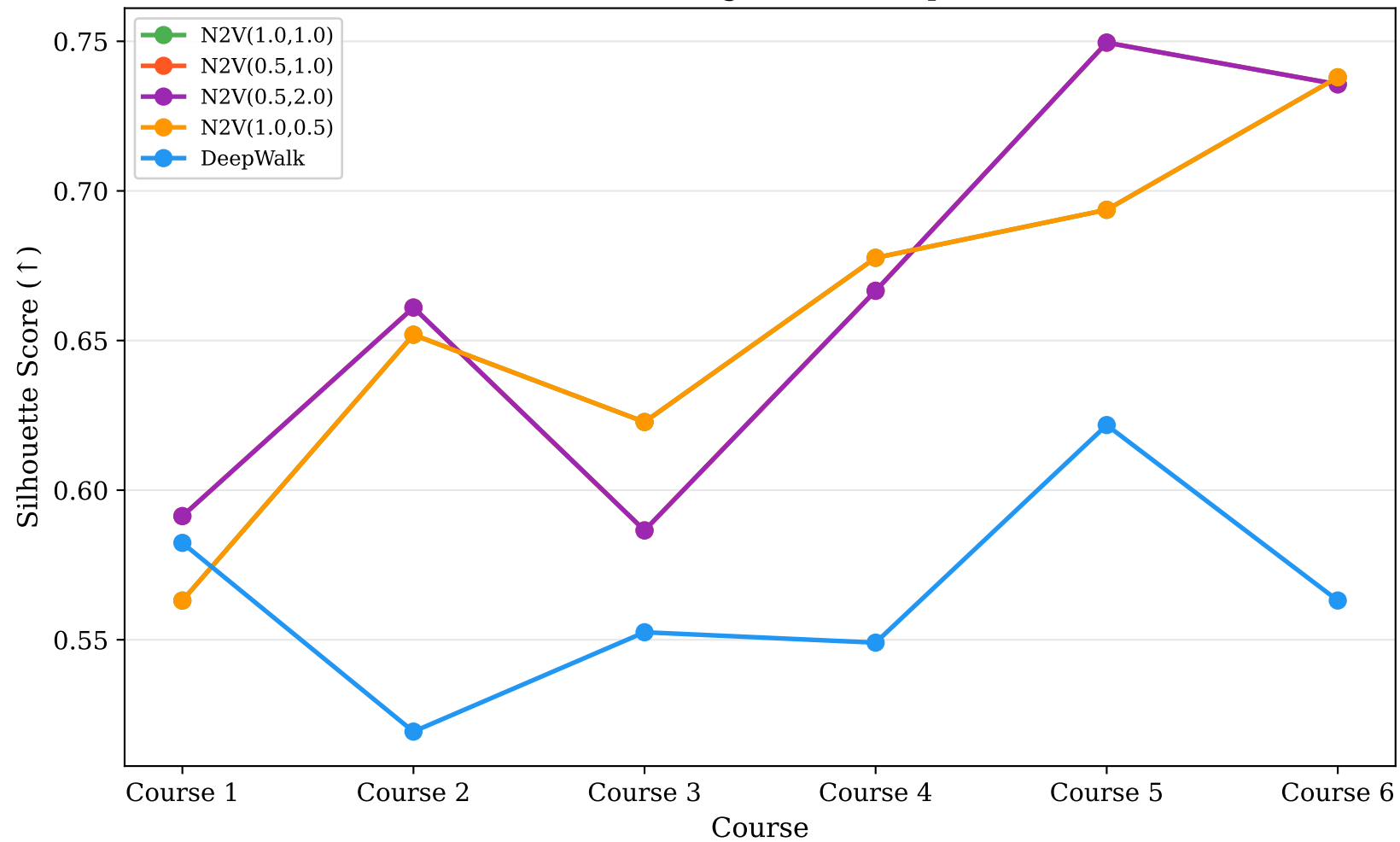
Node2Vec Configuration Comparison
