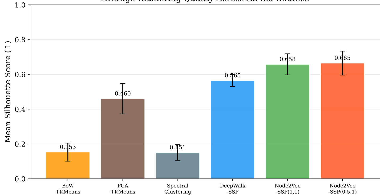
Average Clustering Quality Across All Six Courses
