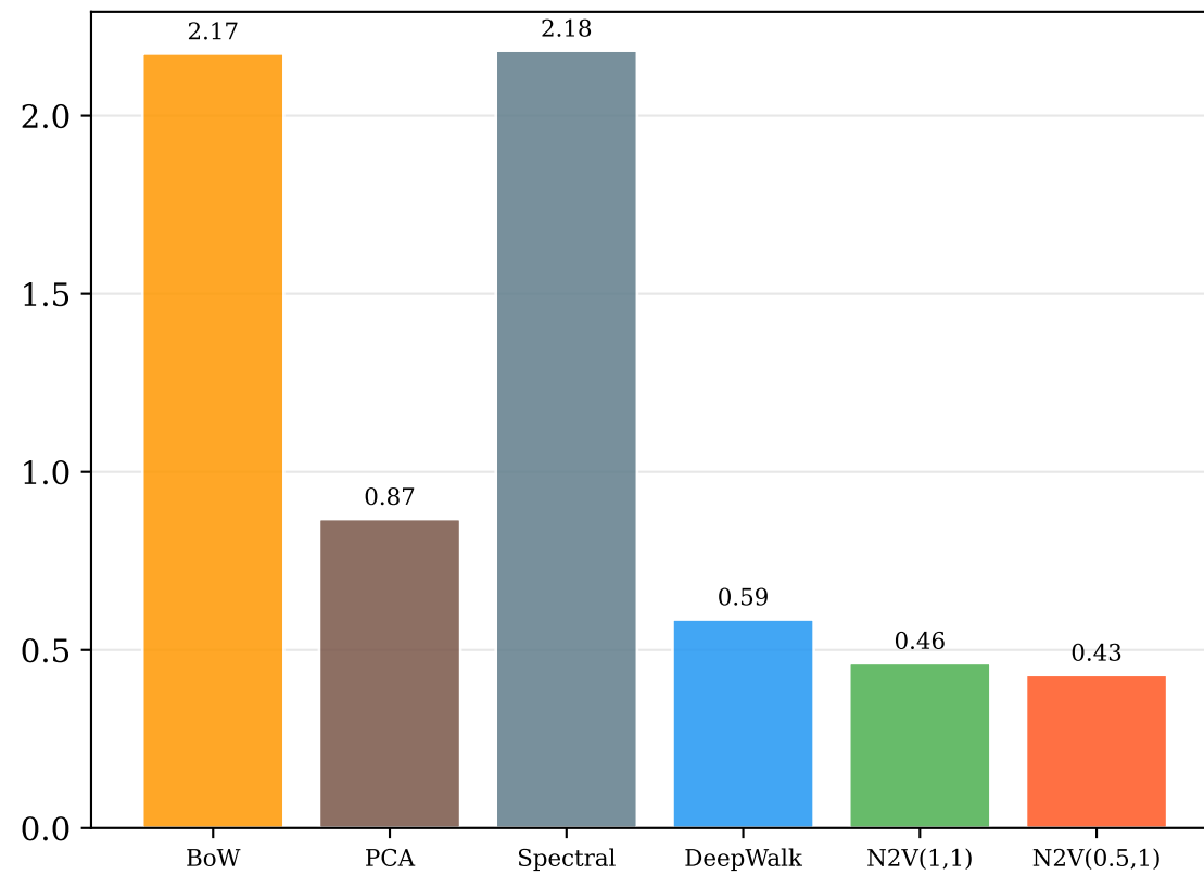
Davies-Bouldin Index (↓)
