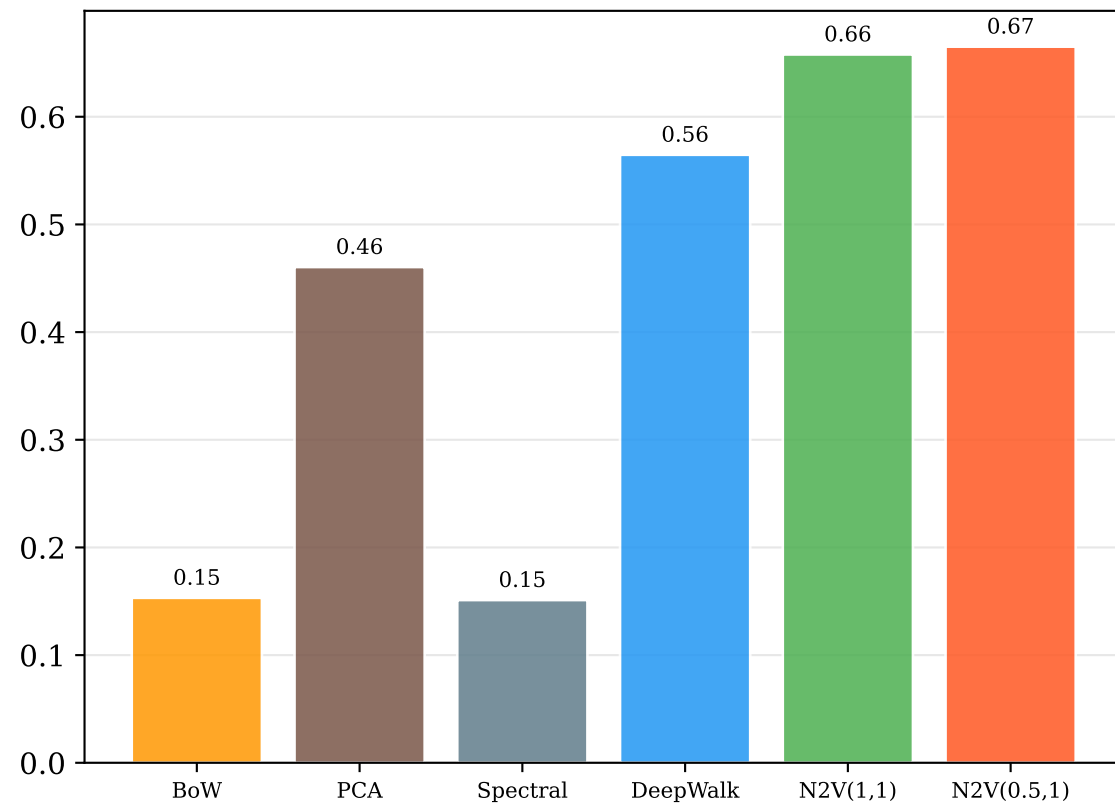
Silhouette Score (↑)
