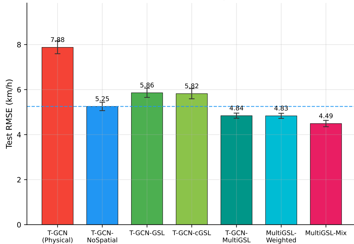
(a) T-GCN family
