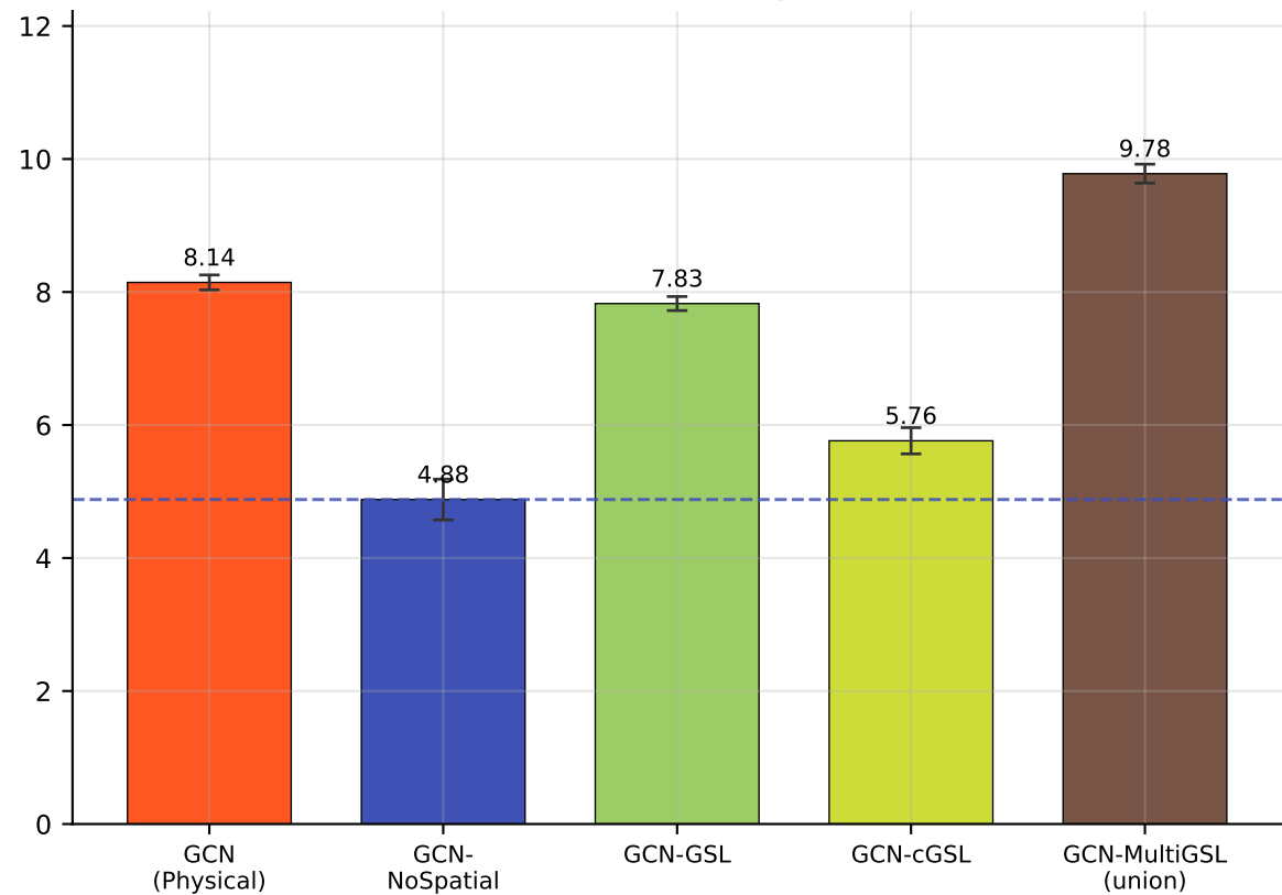
(b) GCN family
