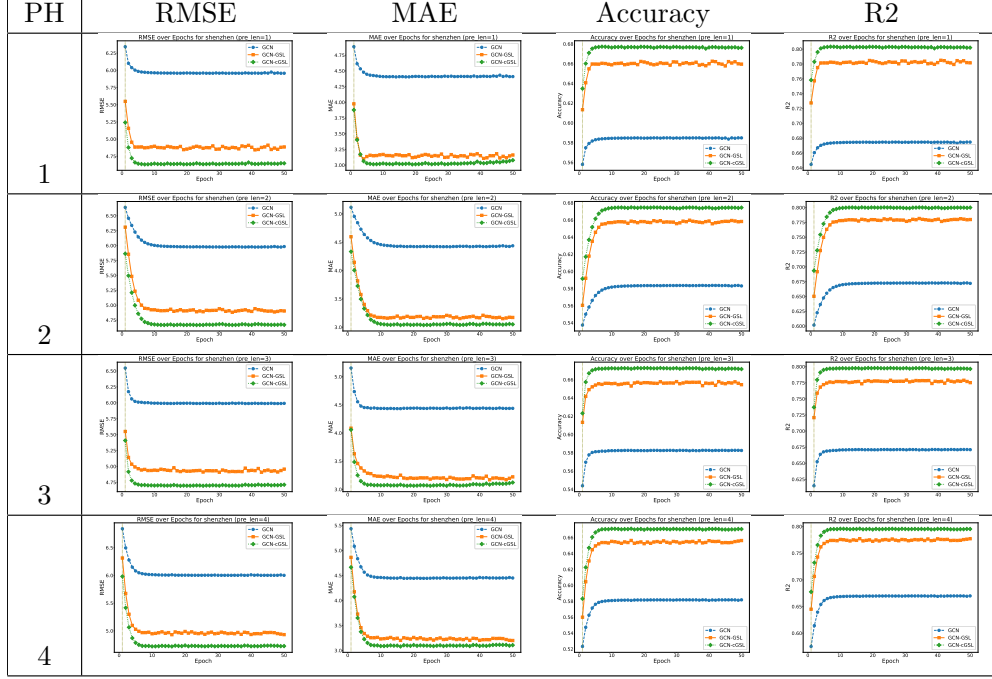
Fig. B1: GCN training on SZ-taxi: GCN-cGSL (green) converges lower than standard GCN (blue).
