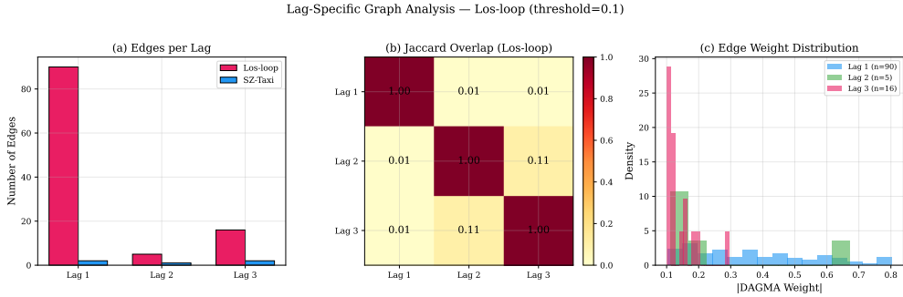
Fig. 2: Lag-specific graph analysis. (a) Edge count per lag for Los-loop and SZ-Taxi ( \tau = 0.1 ). (b) Jaccard overlap between lag-specific edge sets (Los-loop): low overlap confirms structural distinctness. (c) DAGMA weight distributions per lag.
