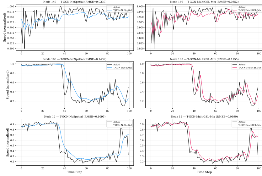
Fig. 4: Predicted vs. actual traffic speed for three high-variance nodes on Los-loop (PH=1, seed=42), 100 consecutive test steps. Both T-GCN-NoSpatial and T-GCN-MultiGSL-Mix predictions closely track the ground truth, with the smooth, slightly lagged character typical of MSE-trained models. Per-node windowed correlations are given in the text.
