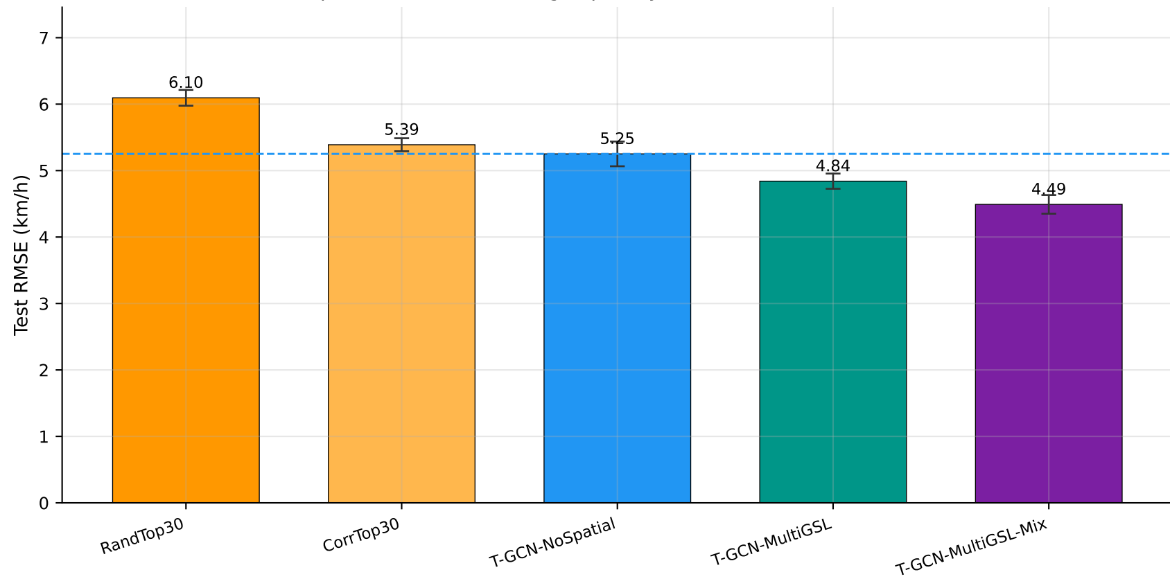
Los-loop PH1: matched 30-edge sparsity controls (five-seed mean \pm SD)
