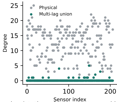
(c) Degrees mean 12.69 vs 0.14
