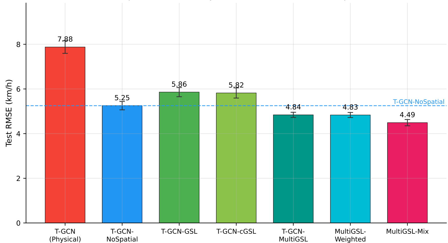
Los-loop PH1: T-GCN family (five-seed mean RMSE \pm sample SD)
