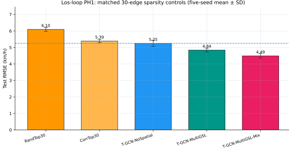
Fig. 6: Matched-sparsity controls on Los-loop at PH1 (five-seed mean \pm sample SD). RandTop30 and CorrTop30 use a 30-edge budget; MultiGSL and Mix use the DAGMA multi-lag graphs. Dashed line: T-GCN-NoSpatial.
