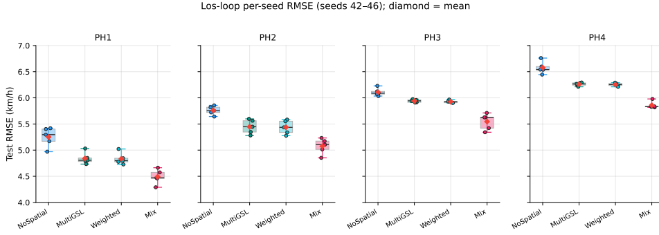
Fig. 7: Los-loop per-seed test RMSE for the multi-lag use ladder (seeds 42–46). Diamonds mark five-seed means matching Table 2.
