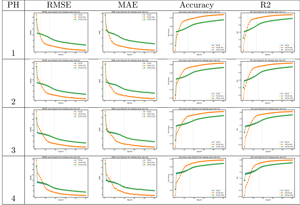
Fig. B4: TGCN training on Los-loop: TGCN-GSL (orange) converges lower than standard TGCN (blue).
