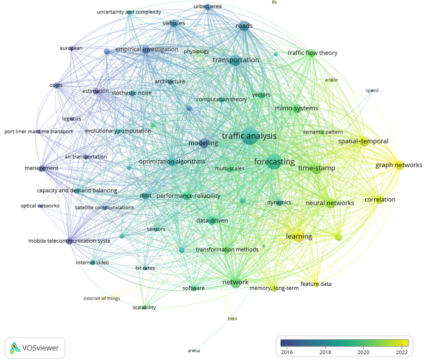
Fig. A1: Clustered keyword co-occurrence network from 784 articles, colored by average publication year. Graph-based methods (right nodes) are the most recent focus.
