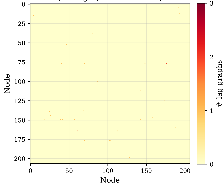
(b) Multi-Lag DAGMA (union) (28 edges, threshold=0.1)
