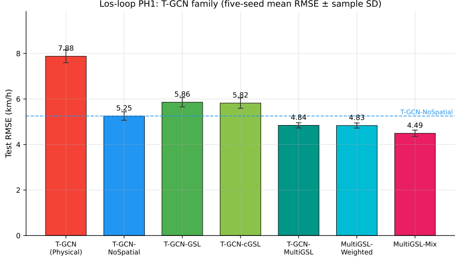
Fig. 3: Los-loop PH1: T-GCN family, five-seed mean RMSE (whiskers: sample SD). Dashed line: T-GCN-NoSpatial.
