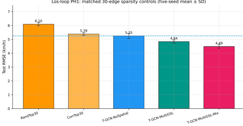
Fig. 7: Matched-sparsity controls on Los-loop at PH1 (five-seed mean \pm sample SD). RandTop30 and CorrTop30 use a 30-edge budget; MultiGSL and Mix use the DAGMA multi-lag graphs. Dashed line: T-GCN-NoSpatial.
