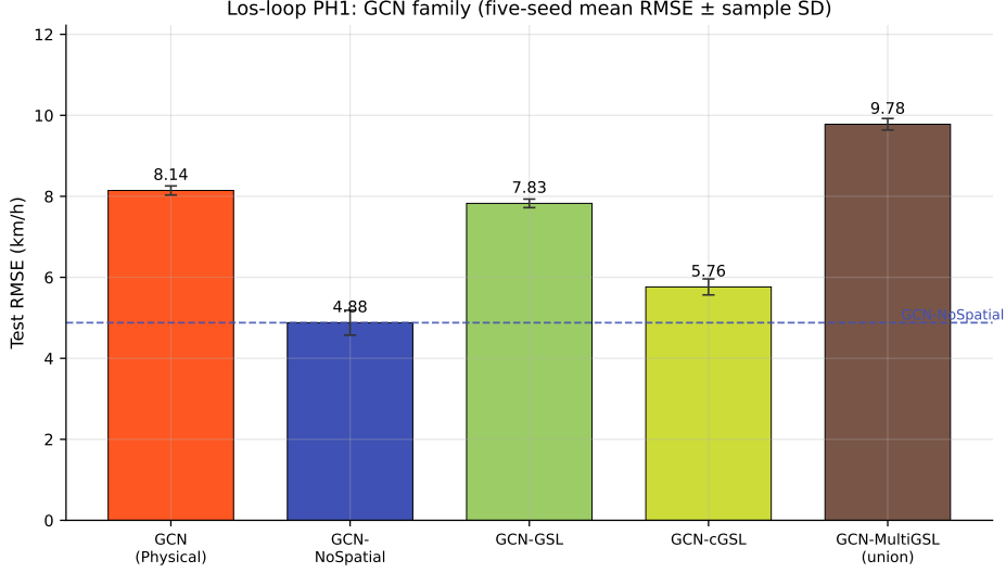
Fig. 4: Los-loop PH1: GCN family, five-seed mean RMSE (whiskers: sample SD). Dashed line: GCN-NoSpatial.
