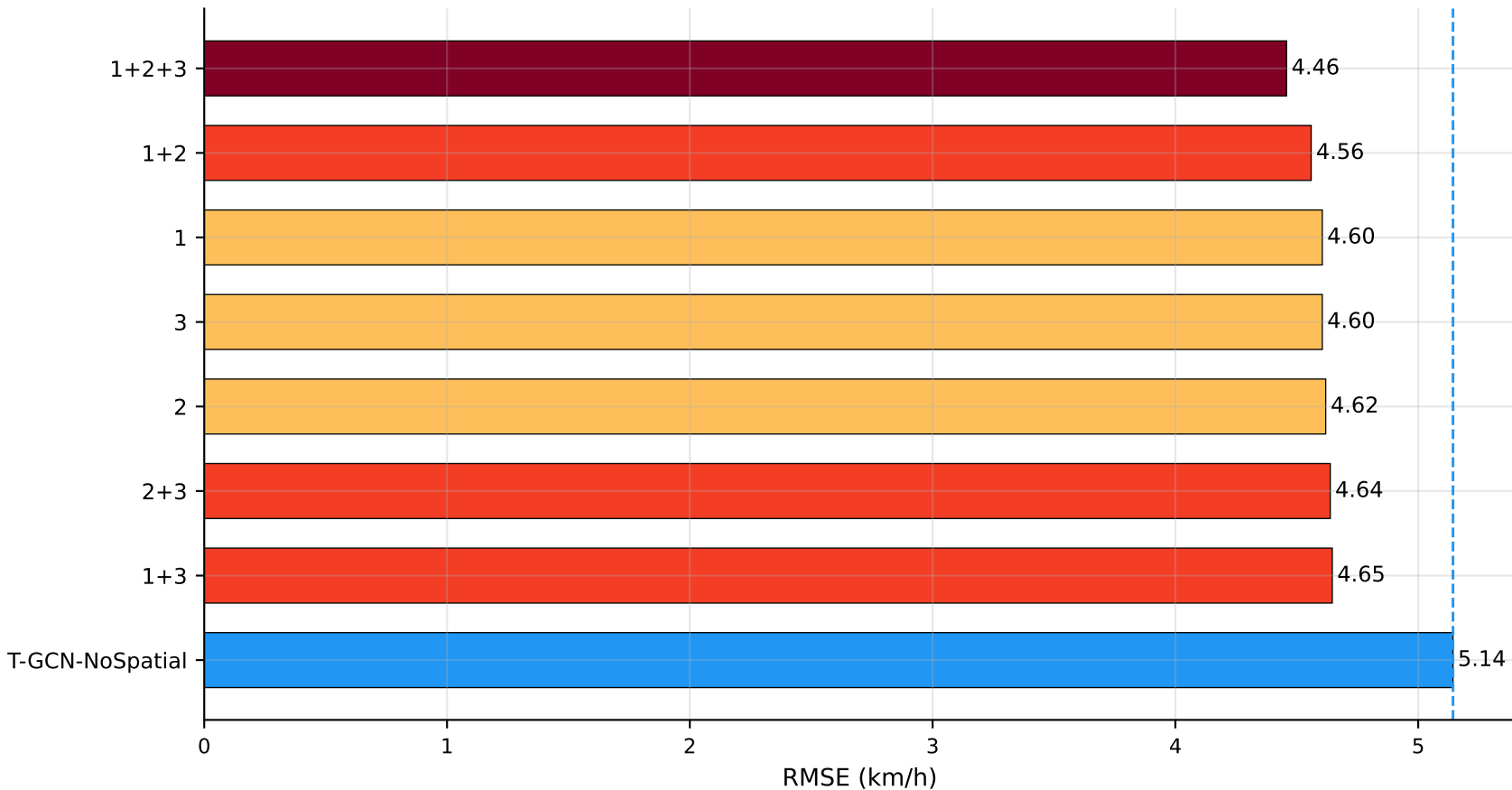
Lag ablation — Los-loop PH1 (seed 42, supplementary)
