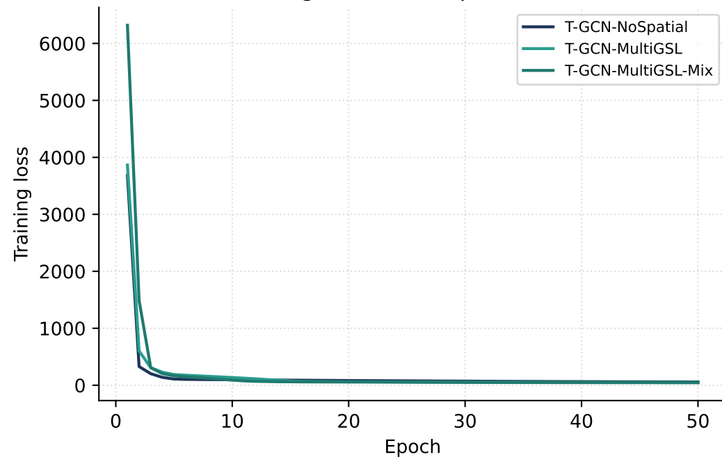
(a) Training loss (Los-loop PH1, seed 42)
