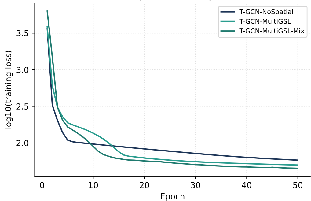
(b) Log-scale training loss
