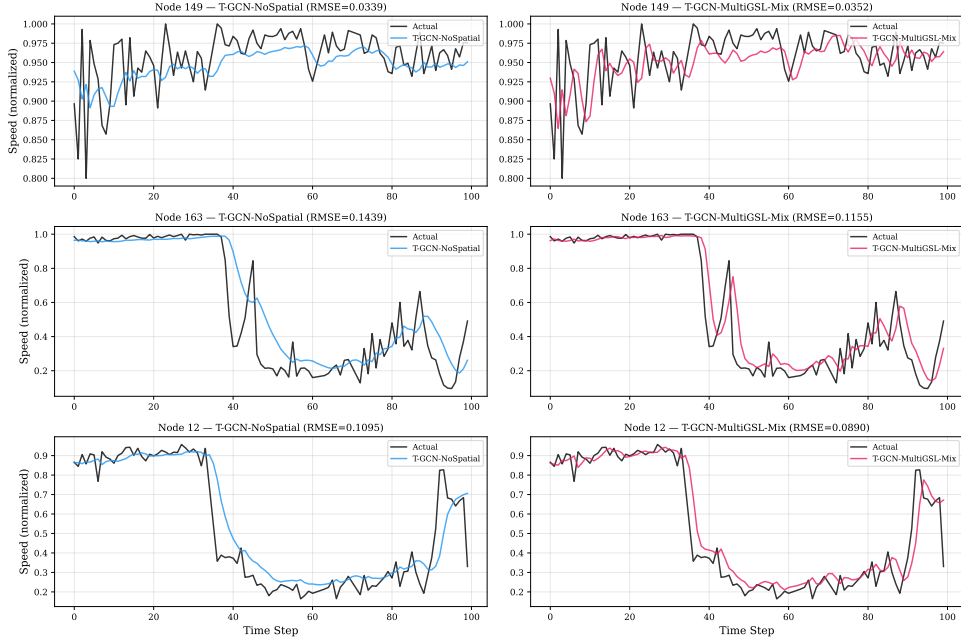
Fig. 6: Qualitative predicted versus actual speed on Los-loop (PH1, seed 42) for three high-variance test nodes (100 consecutive test steps). Left: T-GCN-NoSpatial; right: T-GCN-MultiGSL-Mix. Speeds are on the normalized training scale. Curves are illustrative complements to the aggregate RMSE/MAE tables, not a separate evaluation protocol.
