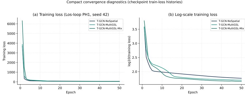
Fig. A2: Compact training-loss histories for T-GCN-NoSpatial, T-GCN-MultiGSL, and T-GCN-MultiGSL-Mix (Los-loop PH1, seed 42). Left: raw loss; right: log-scale. Replaces dense multi-panel convergence grids; not primary evidence for method ranking.
