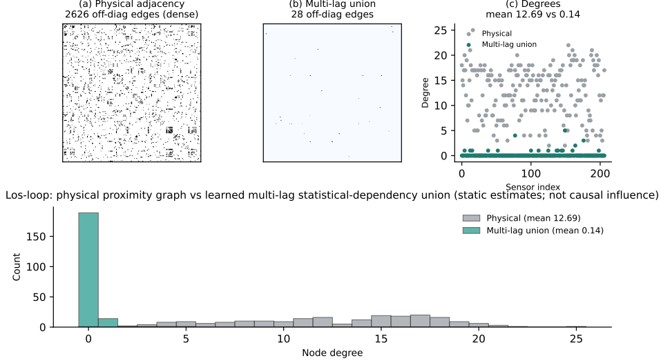
Fig. 7: Los-loop graph structure: (a) physical adjacency (2626 off-diagonal edges; mean degree 12.69); (b) union of multi-lag DAGMA graphs after consumer thresholding (28 edges; mean degree 0.14); (c) node degrees. Learned graphs describe statistical dependency structure.
