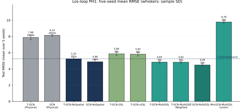
Fig. 4: Los-loop PH1: five-seed mean test RMSE (whiskers: sample standard deviation) for key configurations from the canonical Stage 40 matrix. Annotations show mean RMSE and the learned-edge count ( e ) where relevant. The dashed line is T-GCN-NoSpatial.
