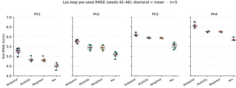
Fig. 5: Los-loop per-seed test RMSE for the multi-lag use ladder (seeds 42–46). Diamonds mark five-seed means matching Table 2.
