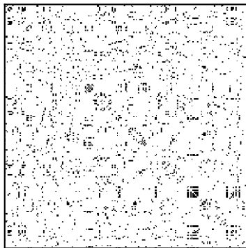
(a) Physical 2626 off-diag edges
