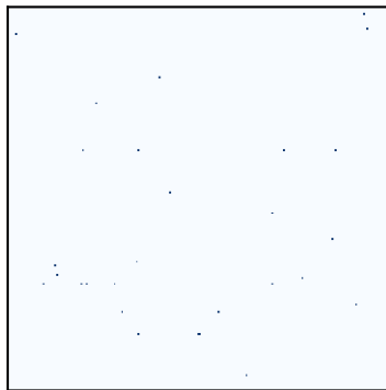
(b) Multi-lag union 28 edges
