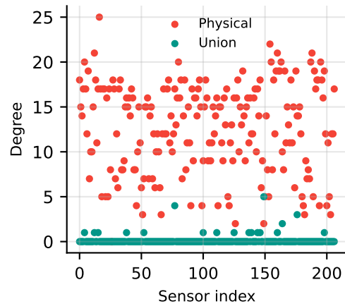
(c) Degrees mean 12.69 vs 0.14
