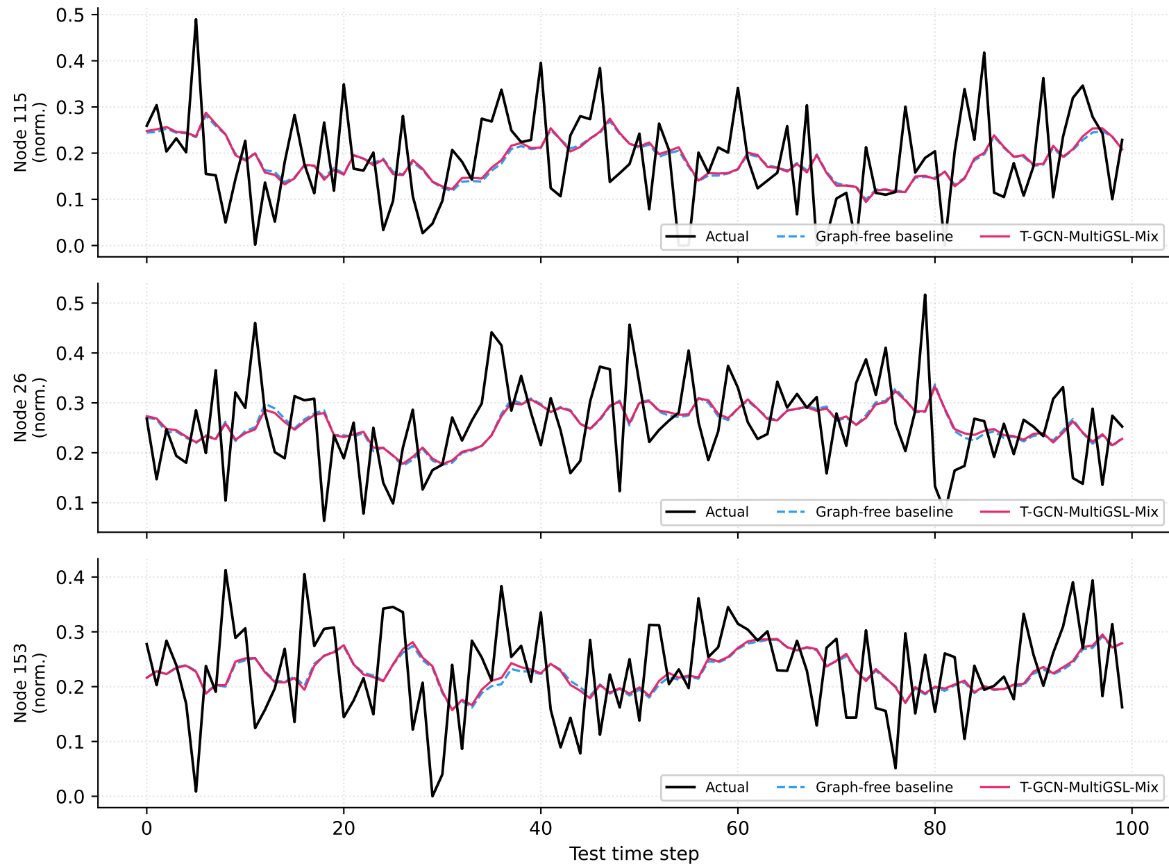
SZ-Taxi PH1, seed 42: predicted vs actual (normalized) three high-variance nodes; 100 consecutive test steps
