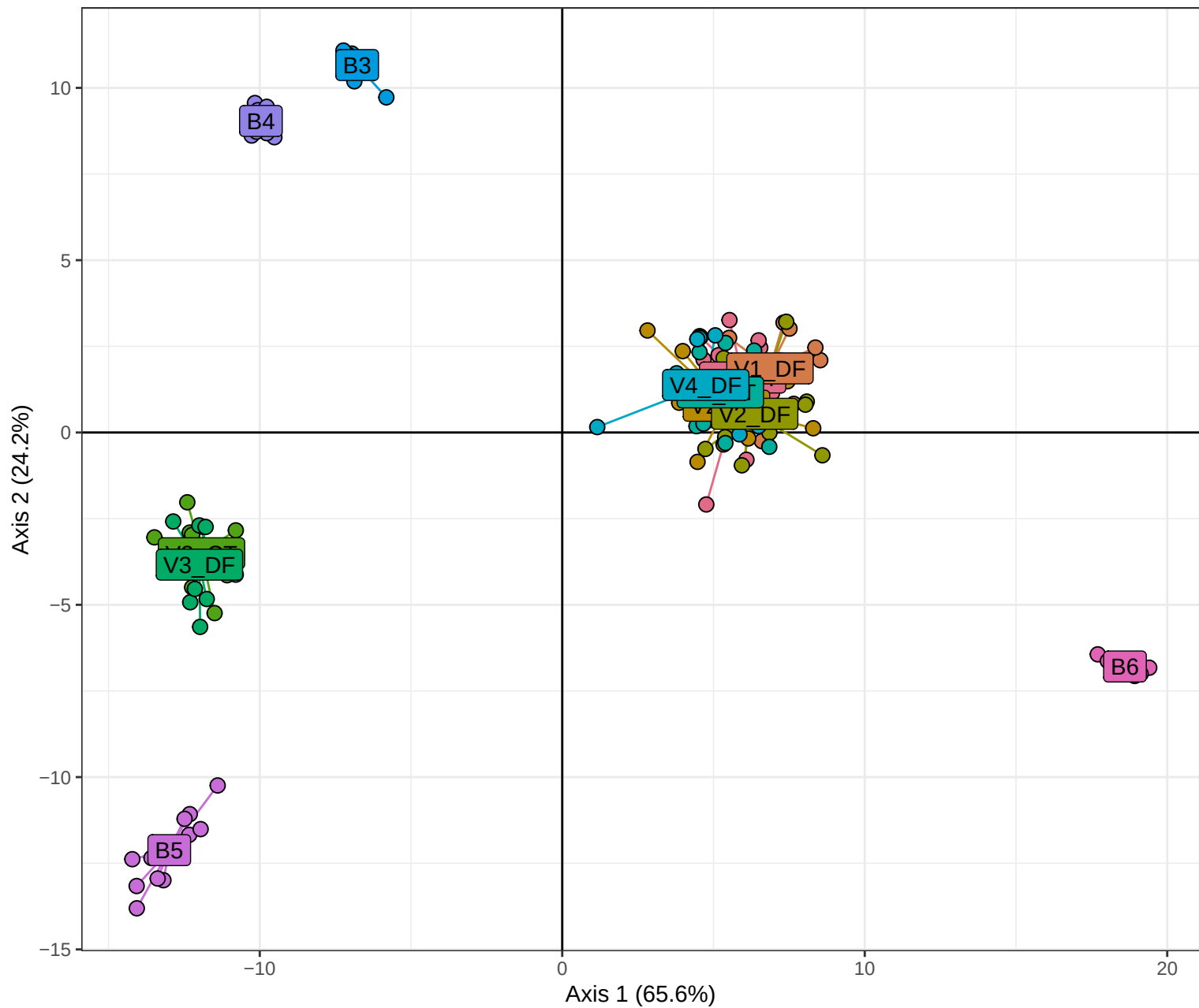
DAPC – haplotypes (3723 haplotypic loci; 8693 haplotypic variants)
