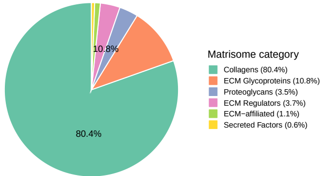
a Matrisome composition (%)
