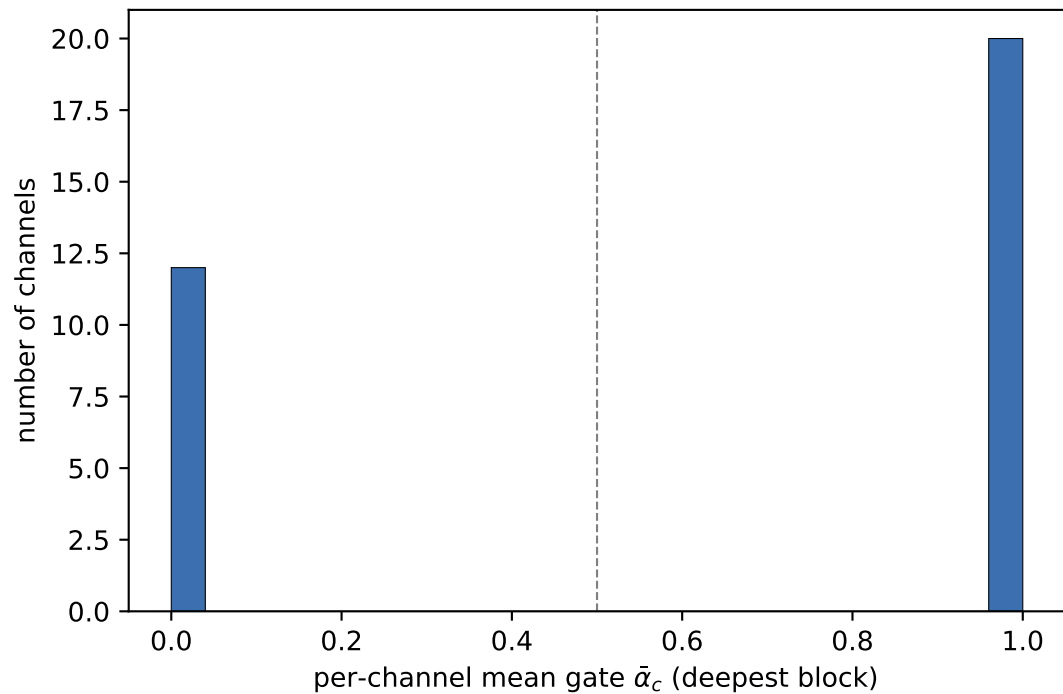
(a) Channel allocation: 20 ch \rightarrow FNO ( \alpha \approx 1 ), 12 ch \rightarrow WNO ( \alpha \approx 0 )
