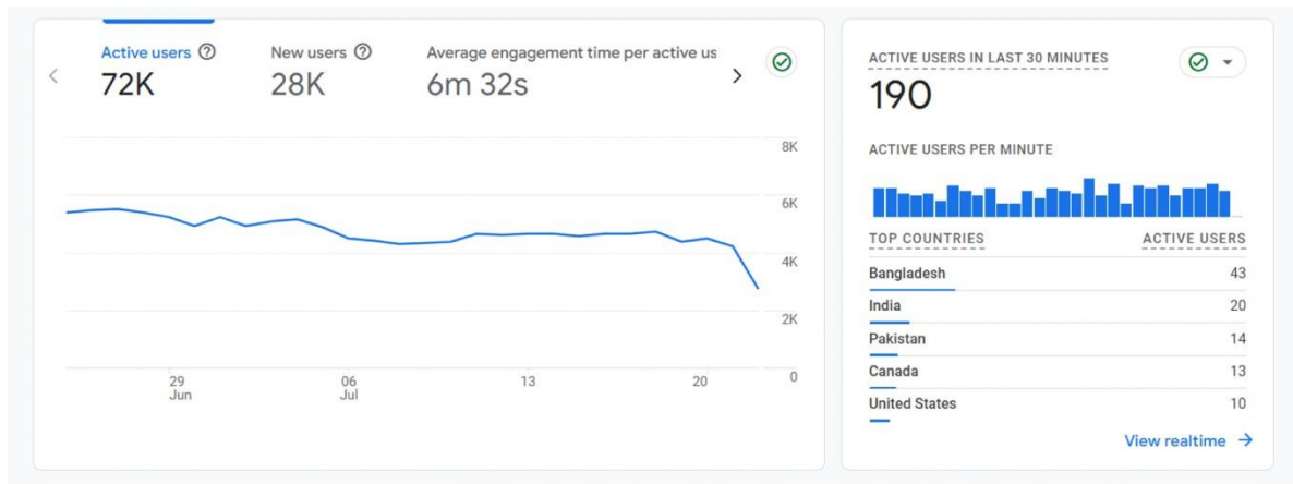
Fig 14: Report overview
