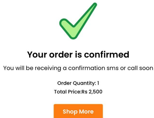
Fig 7: Order Confirmation
