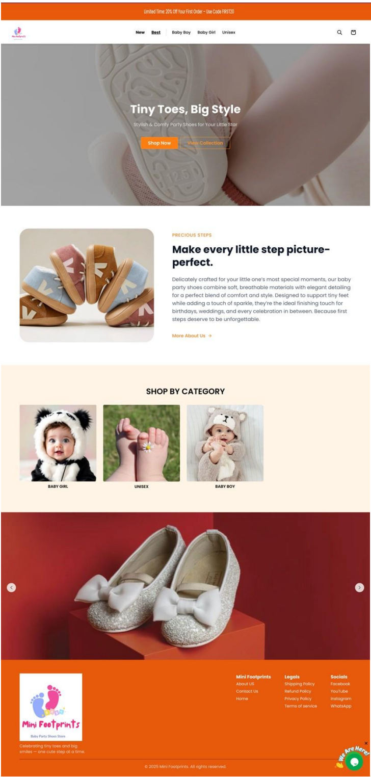
Fig 1: homepage
