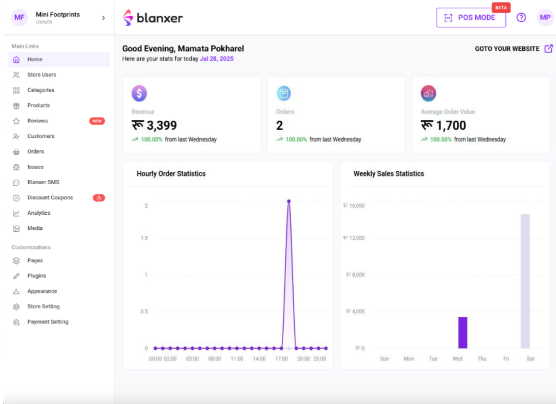
Fig 12: Admin Panel
