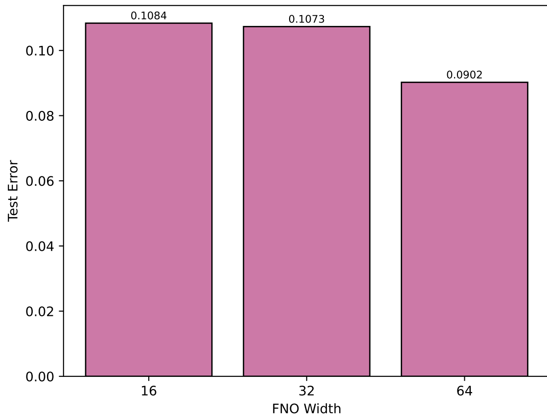
FNO Width Ablation
