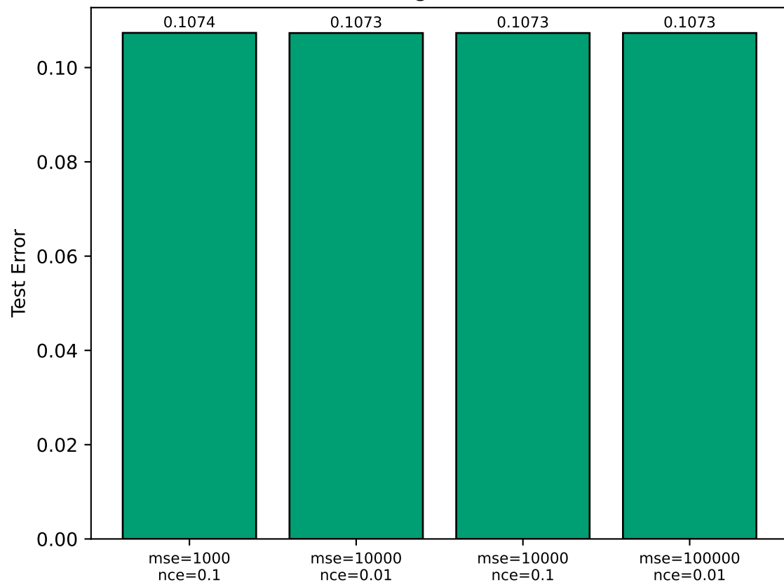
Loss Weights Ablation
