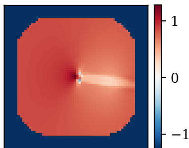
Ground Truth u
