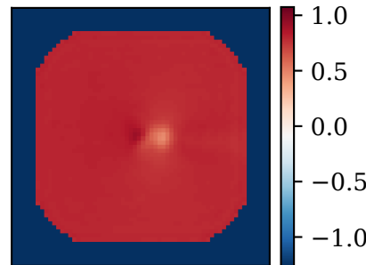
LRR-FNO
