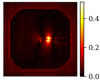
FNO Error
