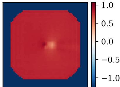
FNO
