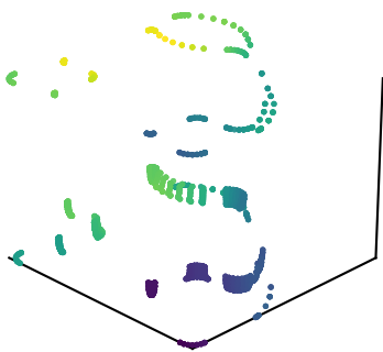
Genus 0 ( \chi=2 )
