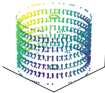
Genus 1 ( \chi=0 )
