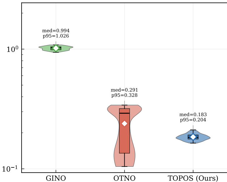
Relative L^2 Error
