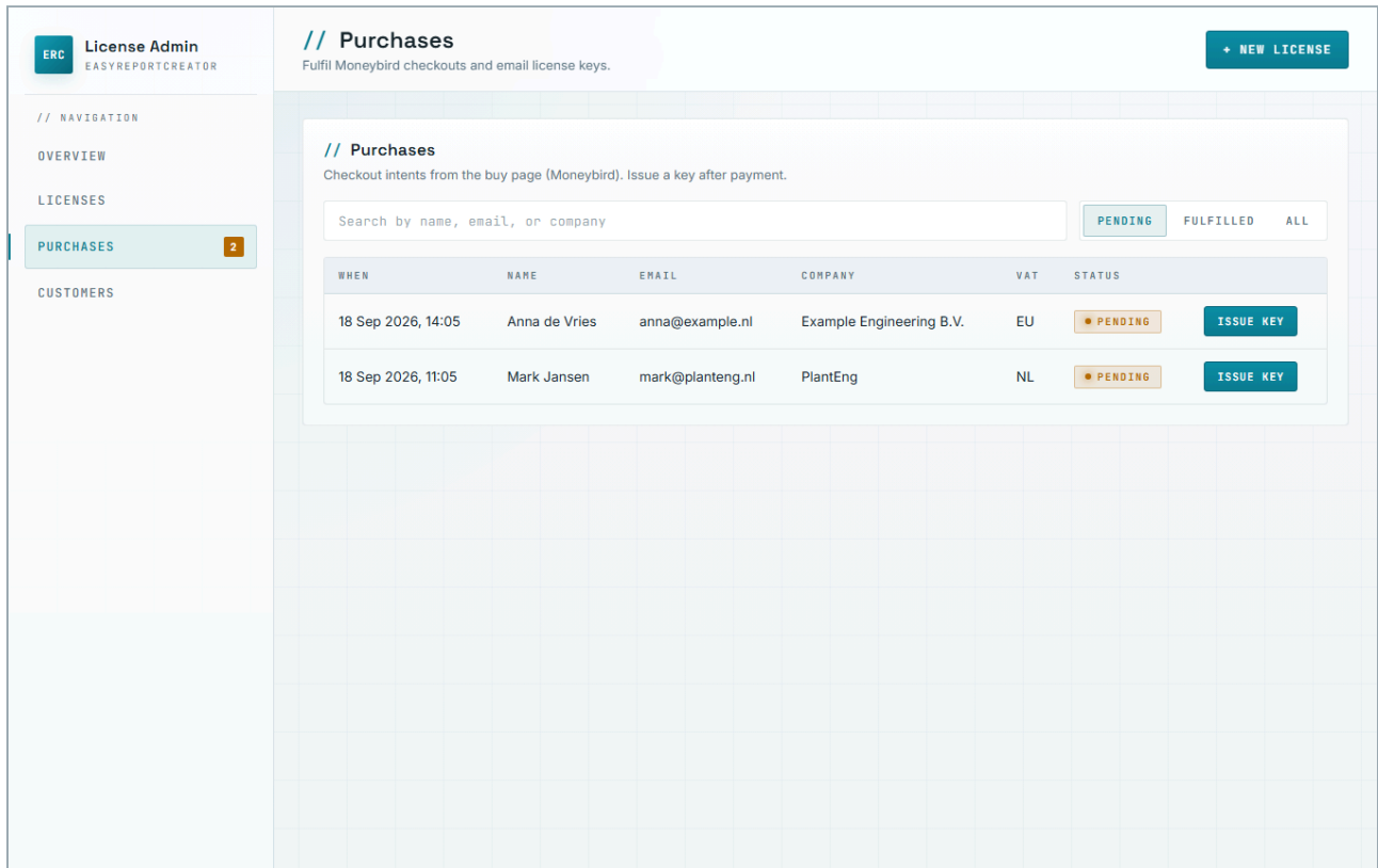
Figure 5. Purchases — pending filter. Issue key creates the licence, marks the intent fulfilled, tries to email the buyer, and copies the key to the clipboard.
