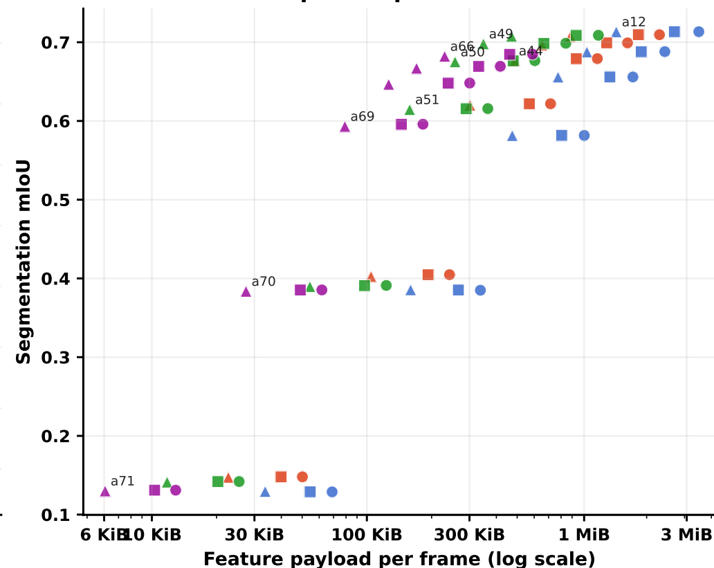
Vehicle/person pixel-class mIoU
