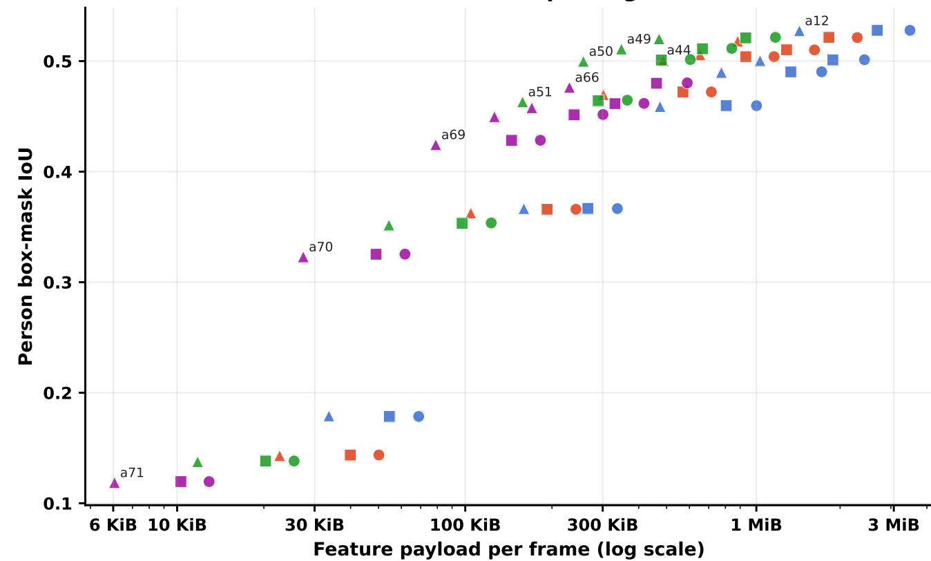
Person localization overlap — higher is better
