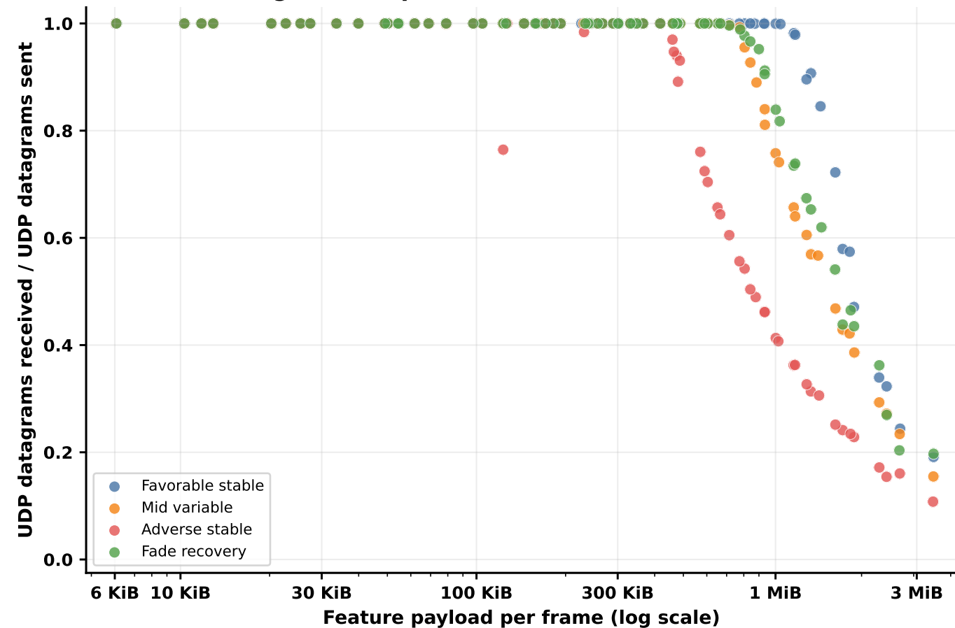
Datagram reception fraction (no retransmission)
