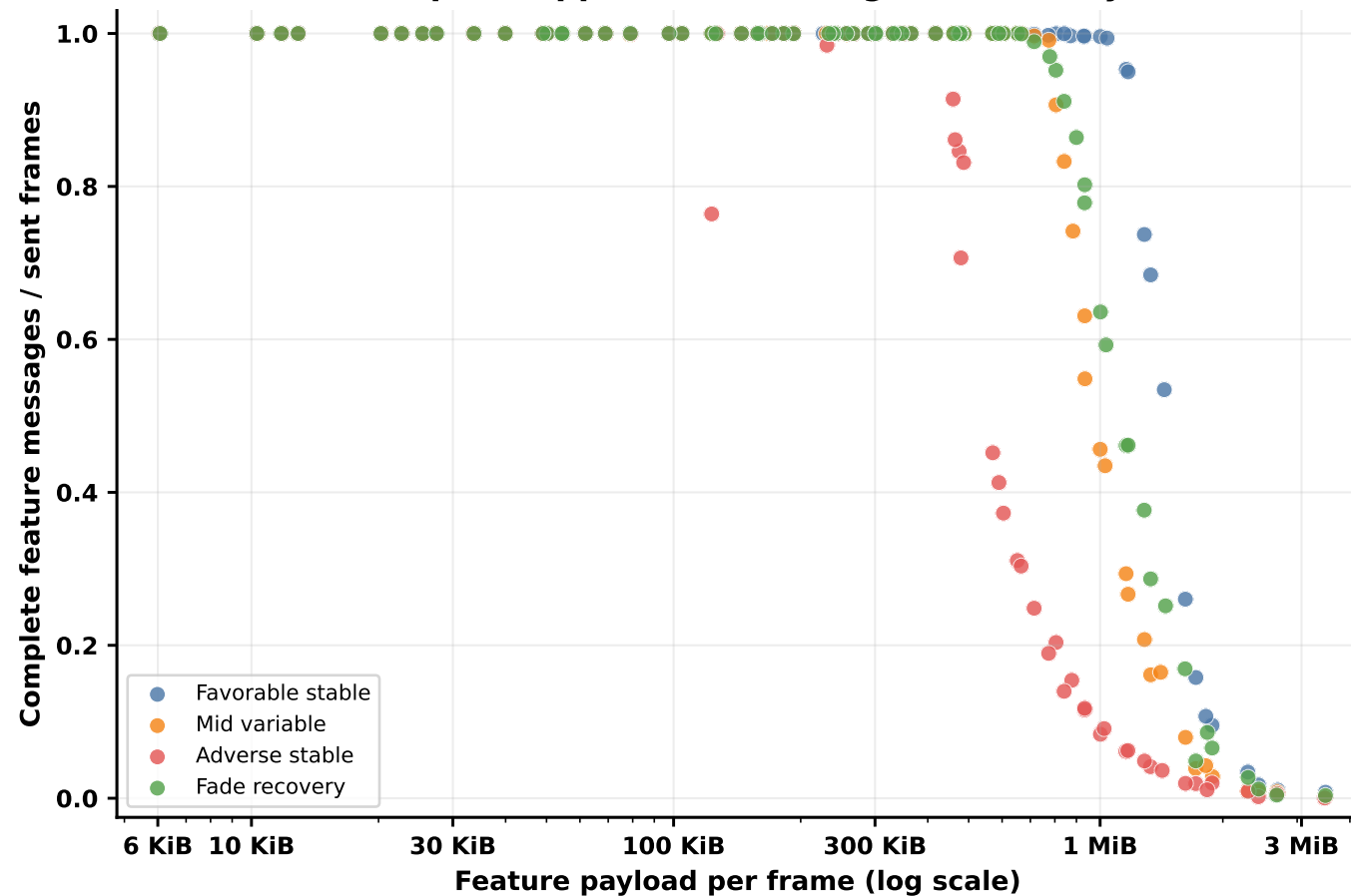
Complete application-message reassembly
